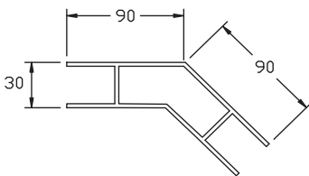
STANDARD 135° MULLION
