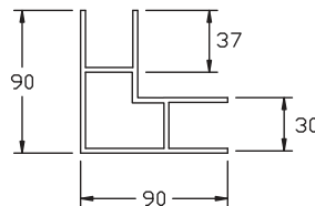
STANDARD 90° MULLION
