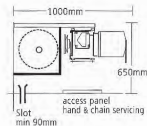
Installation Clearances
